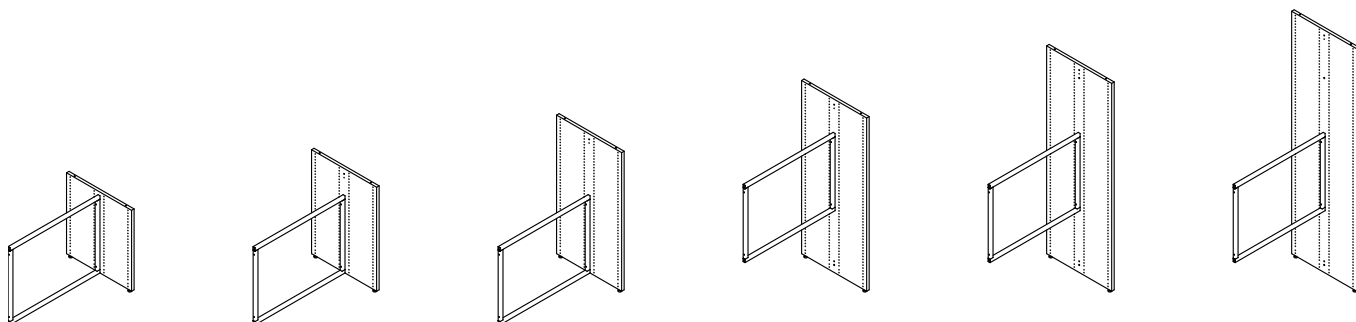
Double-sided add-on bay - H720/920/1220/1520/1820/2120 mm
