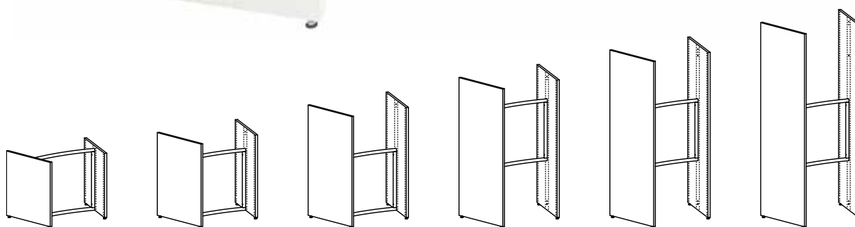
Double-sided starter bay - H720/920/1220/1520/1820/2120 mm
