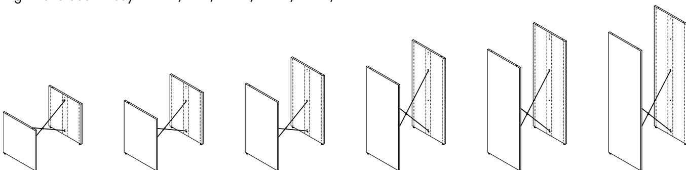
Double-sided starter bay - H720/920/1220/1520/1820/2120 mm
