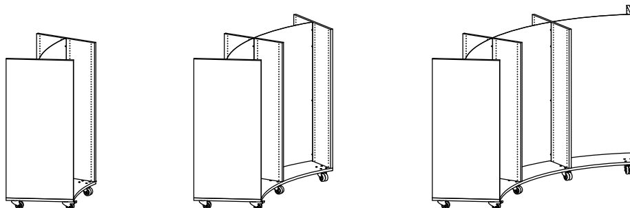
Double-sided H1520 mm - 1/2/3 bays
