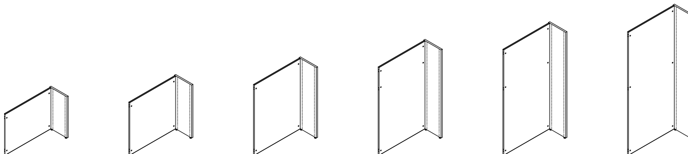
Single-sided add-on bay - H720/920/1220/1520/1820/2120 mm
