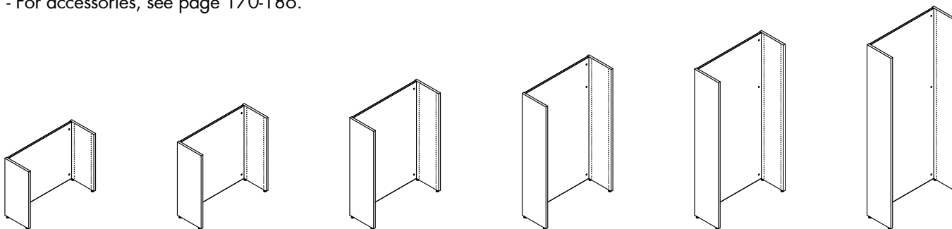
Single-sided starter bay - H720/920/1220/1520/1820/2120 mm
