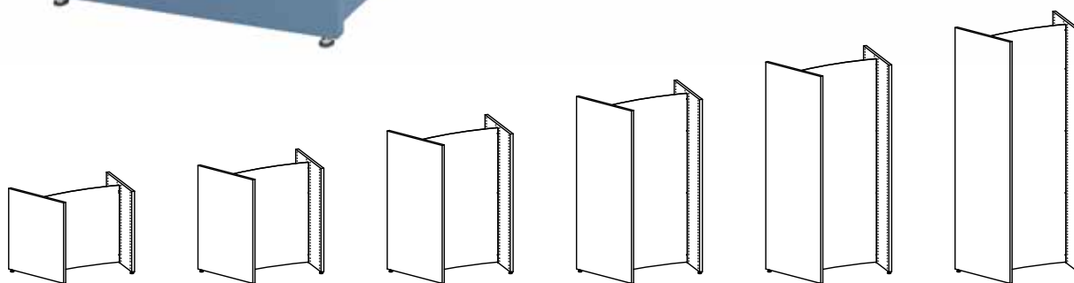
Double-sided freestanding bay - H720/920/1220/1520/1820/2120 mm
